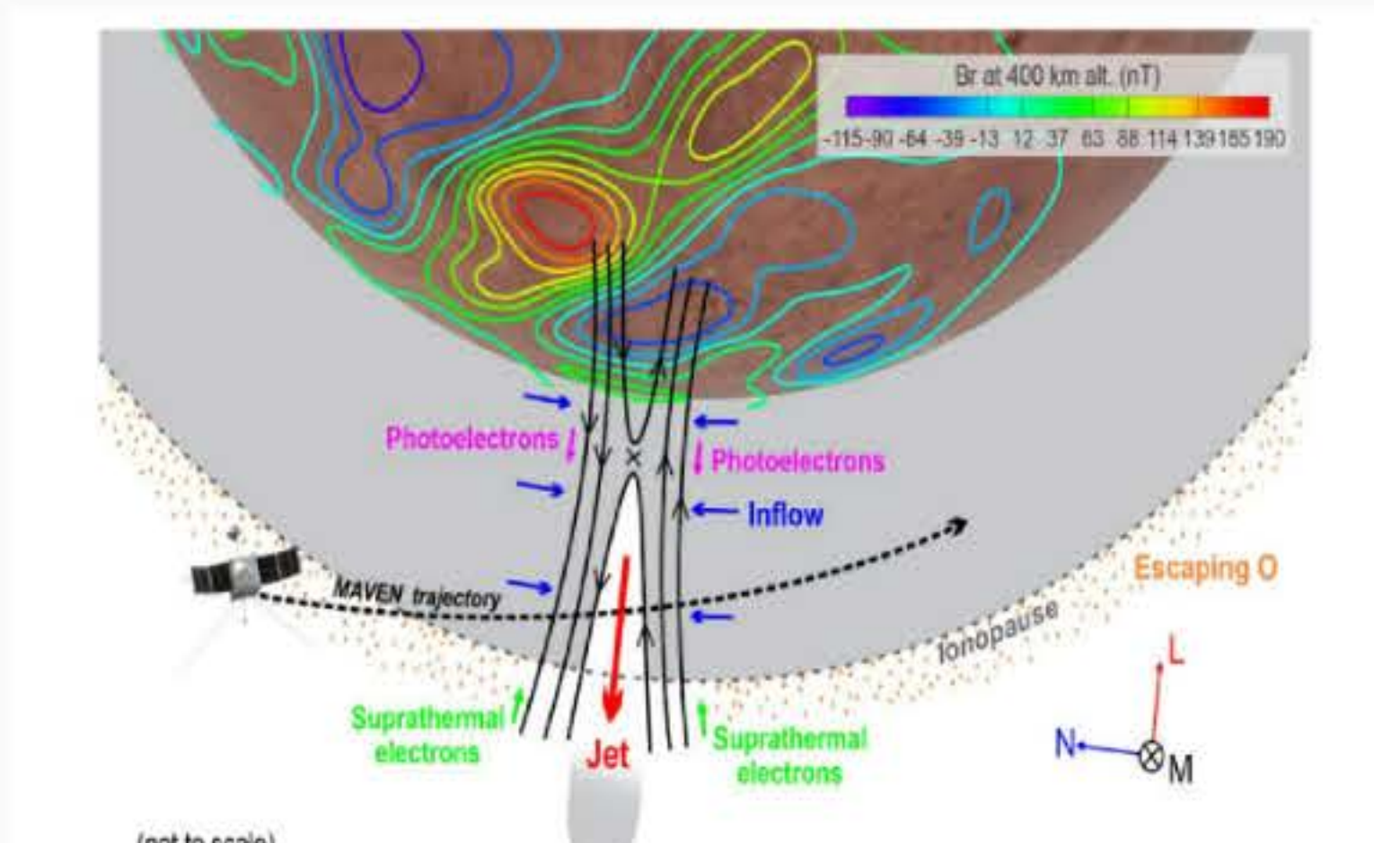
In situ observation of mass ejections caused by magnetic reconnections in the ionosphere of Mars
